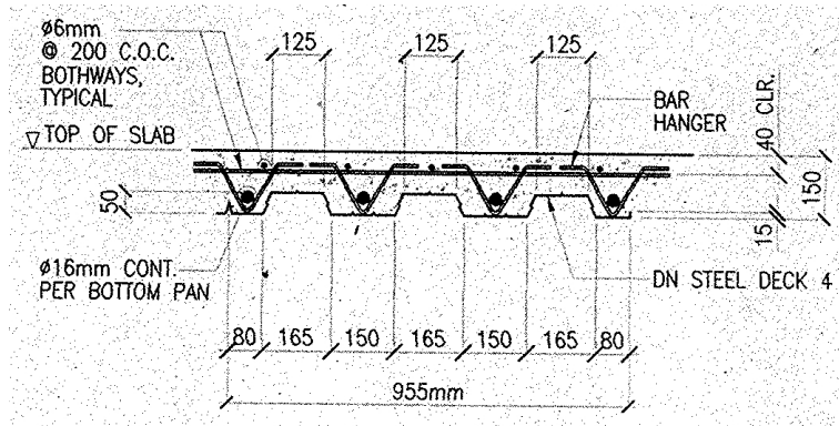
STEEL DECK DETAILS
