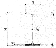
STANDARD BH/BW SECTION
